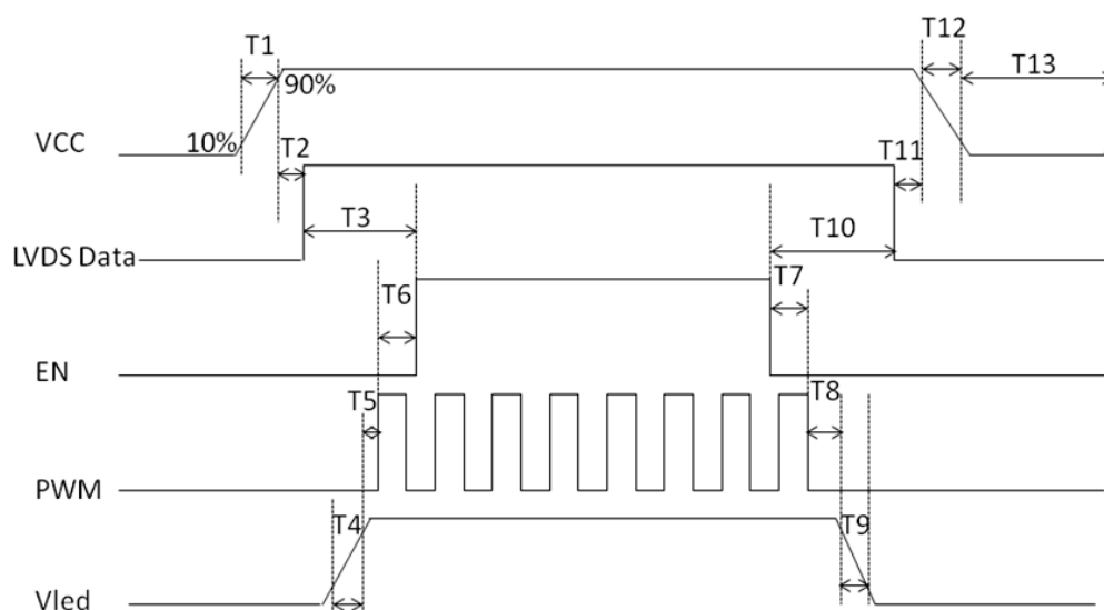
Figure 13 Power Sequence
