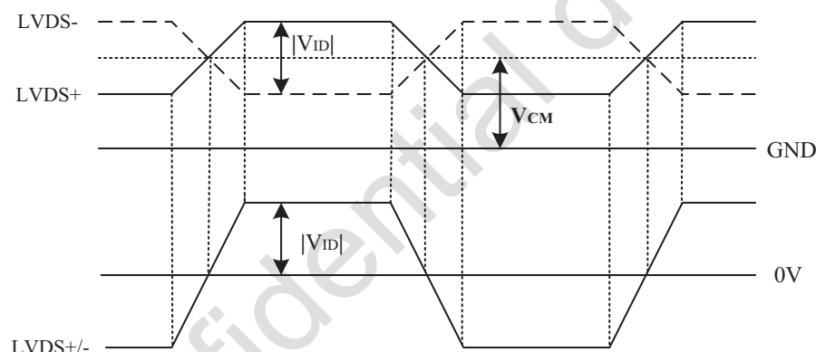
Figure 8 Voltage Definitions
