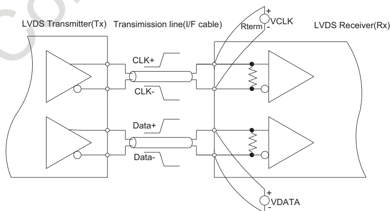
Figure 9 Measurement System
