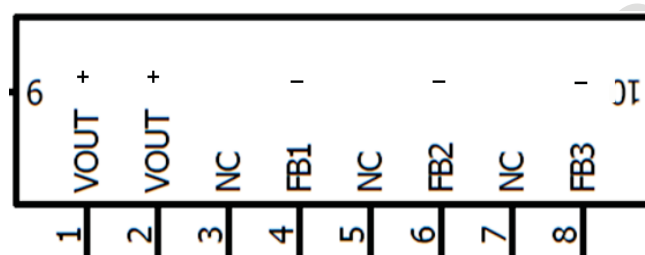
Figure 7 LED Connector
