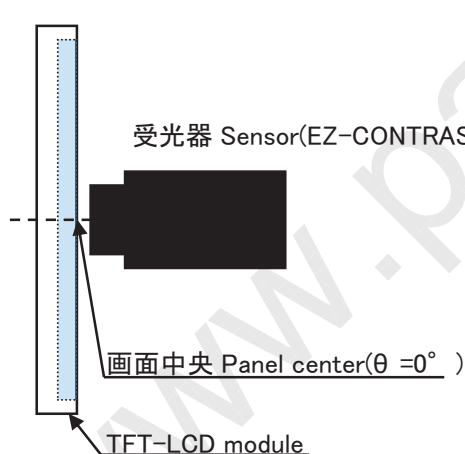
図2-1 視野角特性測定方法 Fig2-1 Measuring setup for Viewing angle
